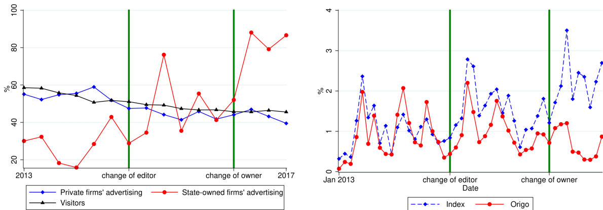
(a) Gov spends more in Origo after capture. (b) Origo covers corruption less after capture
